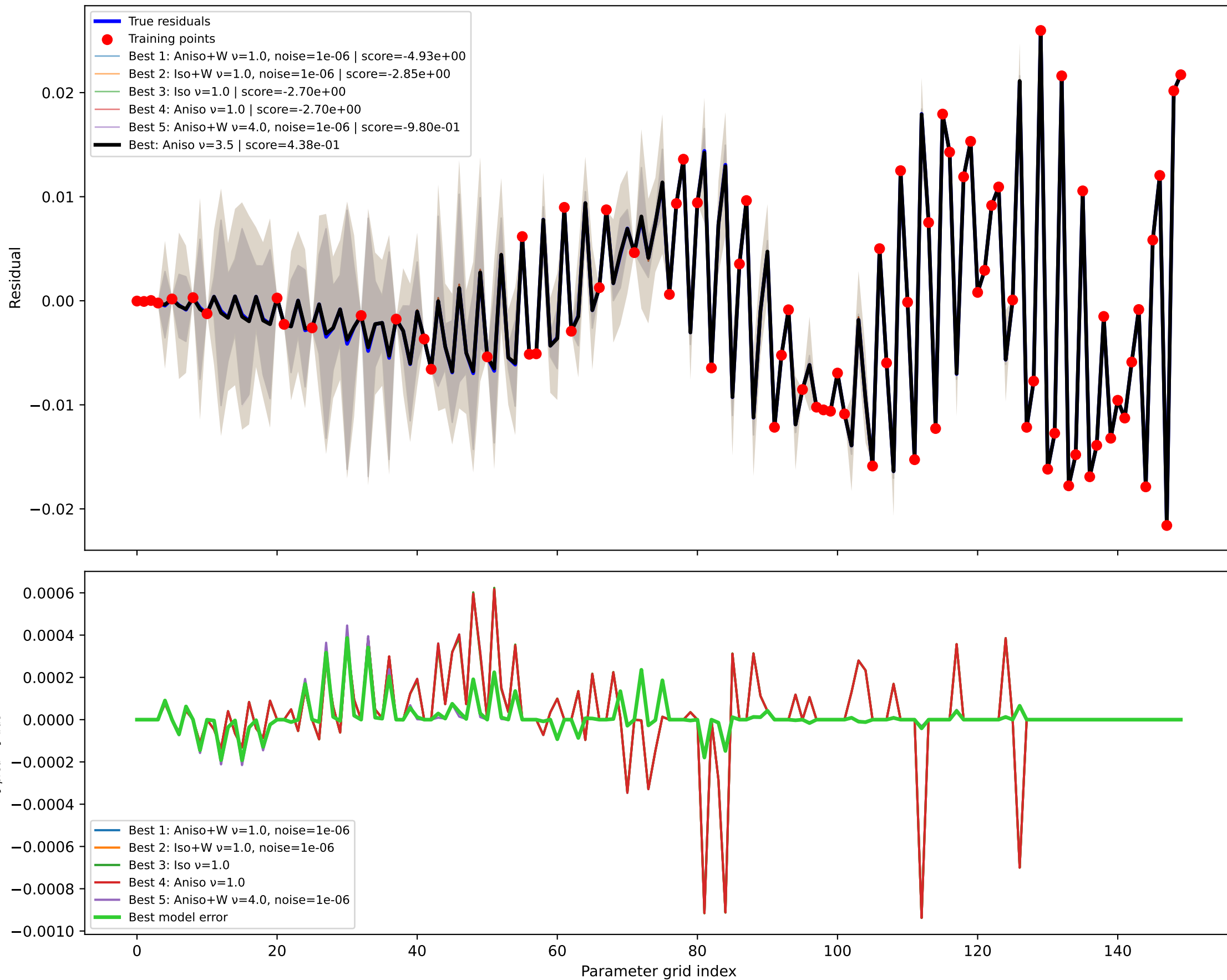
GPR kernel comparison node=44 RMSE=7.651e-05, train RMSE=1.757e-11
